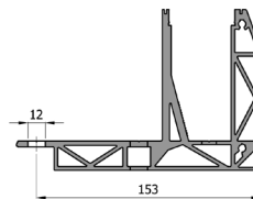
SECTION B-B (1:2.5)
