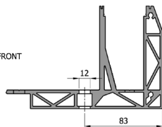
SECTION A-A (1:2.5)
