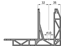
SECTION C-C (1:2.5)
