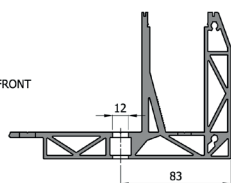
SECTION A-A (1:2.5)
