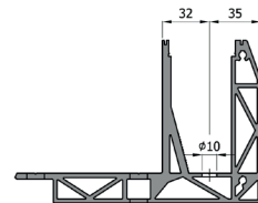
SECTION C-C (1:2.5)
