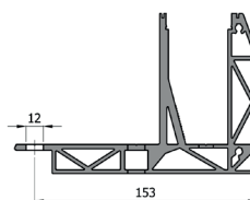
SECTION B-B (1:2.5)
