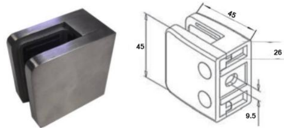
KLH10F-45/45-Zintec St/St Effect - 10mm Glass Zamack Glass Clamp (No Pin)
