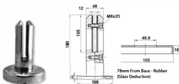
GLH1080 Round Spigot & Base (Rubbers for 10 and 12mm) 316G Satin and Mirror
