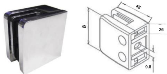
KLH10F-45/45-M Zamack Mirror Finish - 10mm Glass (No Pin)
