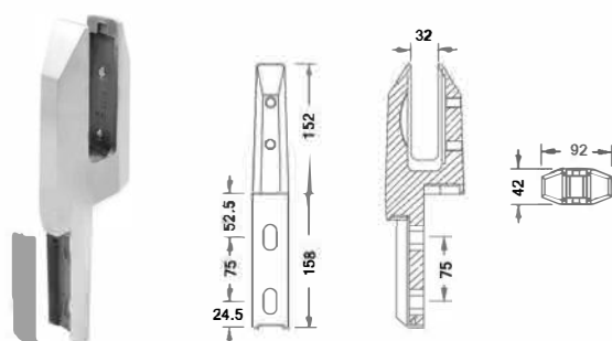
KT-Tilt-Lock Duplex Stainless Steel 2205 Satin Finish 12-25.52mm Glass
