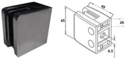
KLH10F-45/45 Satin Finish - 10mm Glass (No Pin) 304
