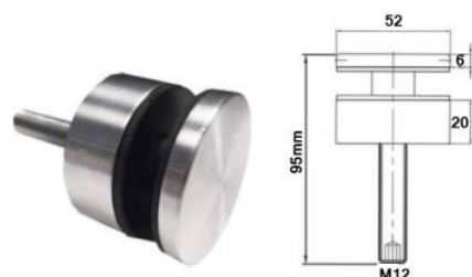
JK-1015 Solid Threaded Body – Flat Head M12 Removable Thread 304/316
