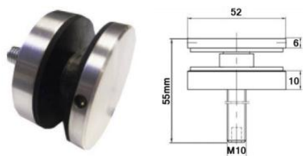
JK-1014 Solid Threaded Body – Flat Head M10 Removable Thread 304/316
