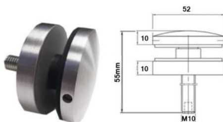
JK-1017 Solid Threaded Body – Convex Head M10 Removable Thread 304/316
