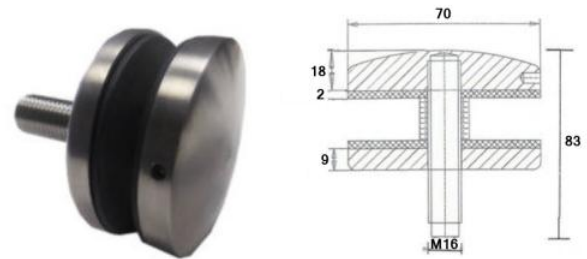
GLH1070-M16 70mm Face - M16 Removable Thread 316
