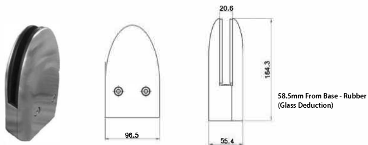
GLH1081 Novo Spigot (12mm Glass) 316G Satin
