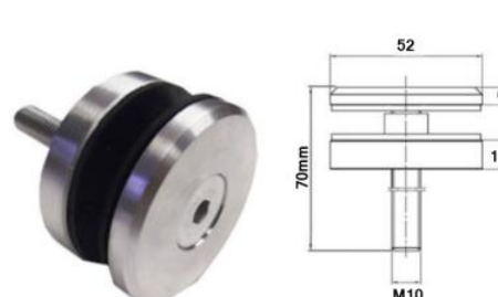
JK-1012 Solid Threaded Body – Screw Head M10 Removable Thread 304/316
