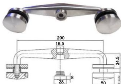
GLH1030 Glass Retainer - Flat 316
