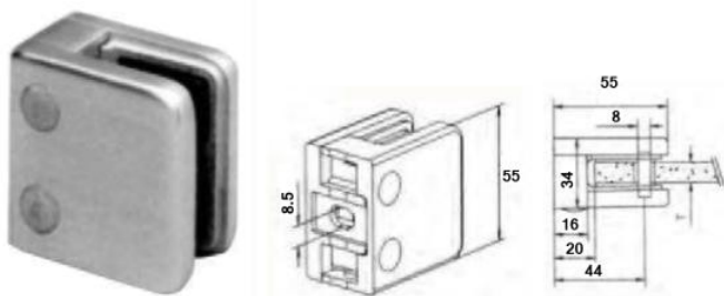
KLH12F 304/316G Satin/Mirror Flat - Square 55 x 55mm 304/316
