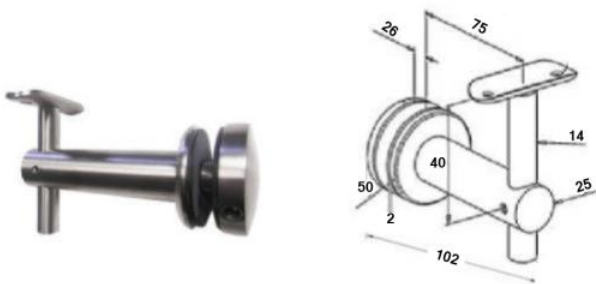
HH1015K-75 Convex Head - Glass to Handrail 304/316
