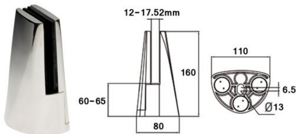
CC-780-BA(Mirror) CC-780-S(Satin) Base Spigot - 12, 15 & 17.52mm Glass
