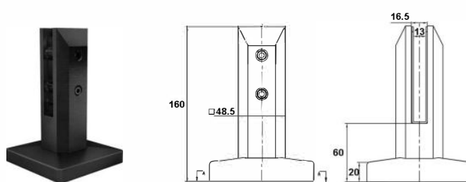
KT-Spigot-Black PVD Coated Black Spigot To Suit 10-12mm Glass
