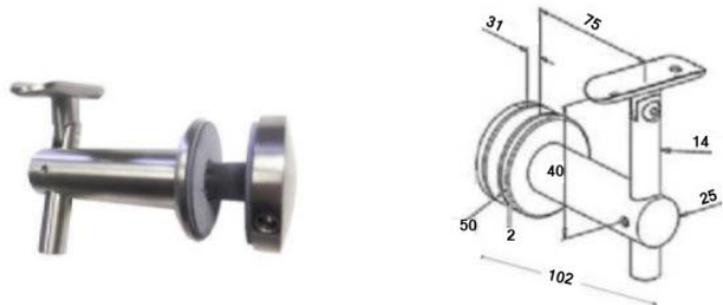
HH1015-75-ADJ Convex Head - Glass to Handrail 304/316
