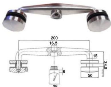
GLH1031 Glass Retainer - 48/50mm Tube 316
