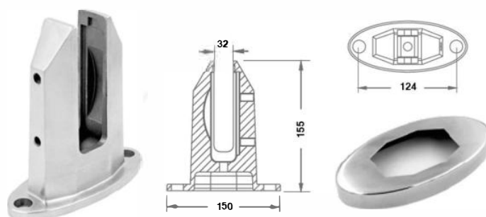
KT-Spigot-Tilt Duplex Stainless Steel 2205 Satin Finish 12-25.52mm Glass
