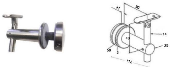
HH1015-90-ADJ Convex Head (Adjustable) - Glass to Handrail 304/316
