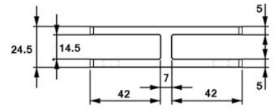
KLH10-STIFF-180 Duplex Stainless Steel – Satin Finish 10-12mm 180 Degree Glass Stiffener
