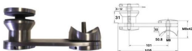
GLH1011K-50.8 Single Glass Retainer (50 x 50mm) 316
