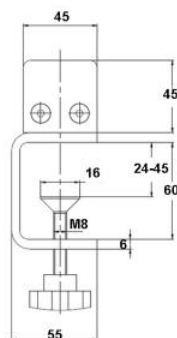
KT-Sneeze-Screen-Clamp 304 Grade To Suit 6 / 8 / 10mm Glass
